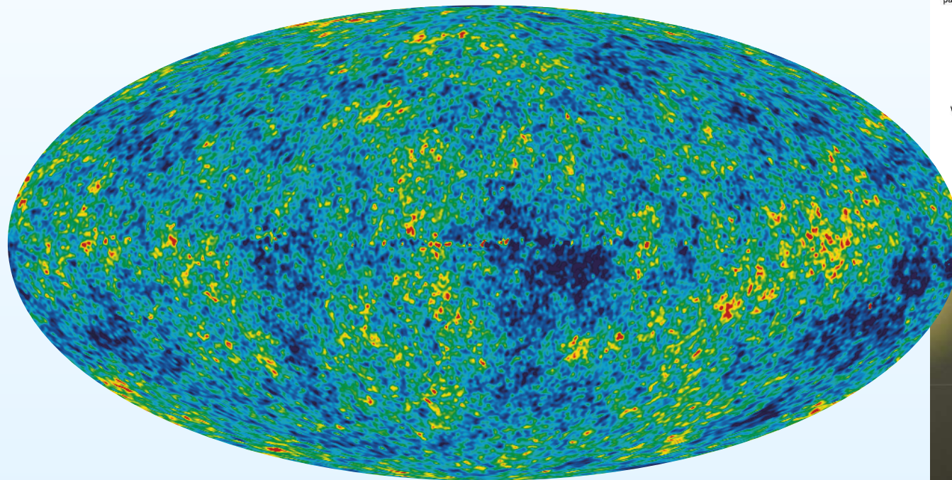
-200 T( \mu K) +200 WMAP 5-year
