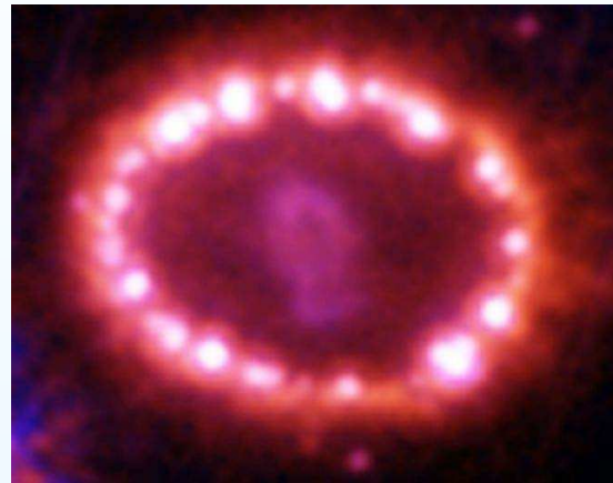
supernova 1987A
