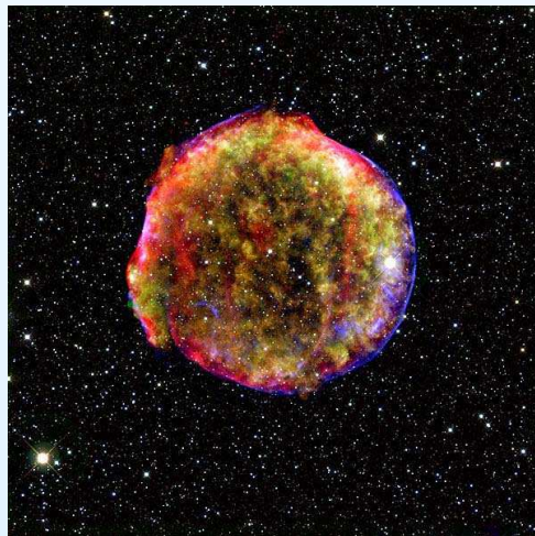
Tychonova supernova (1572)
